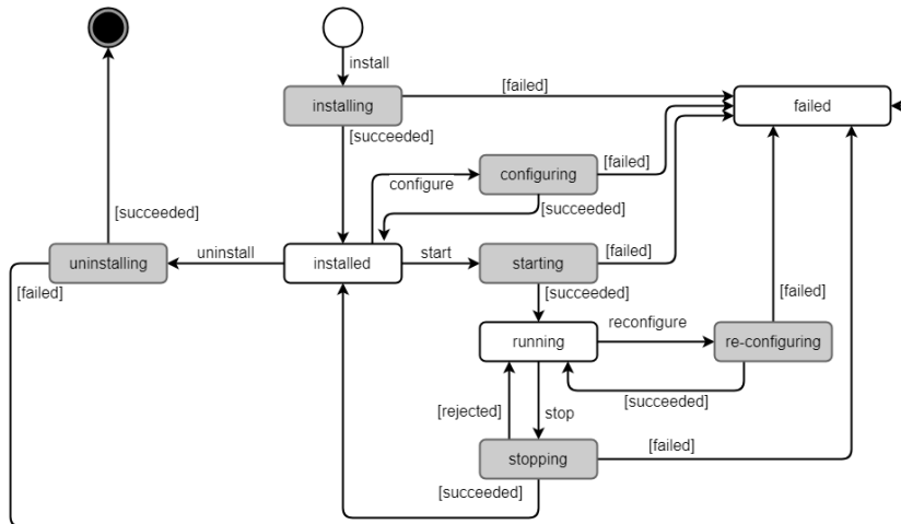
Figure 1: A sample application lifecycle graph.
