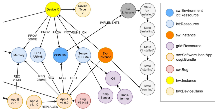
Figure 4: Subset of a knowledge graph stored in the Knowledge-Based Software Management backend.
