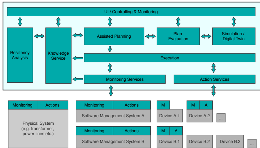
Figure 3: KBSM Framework.
